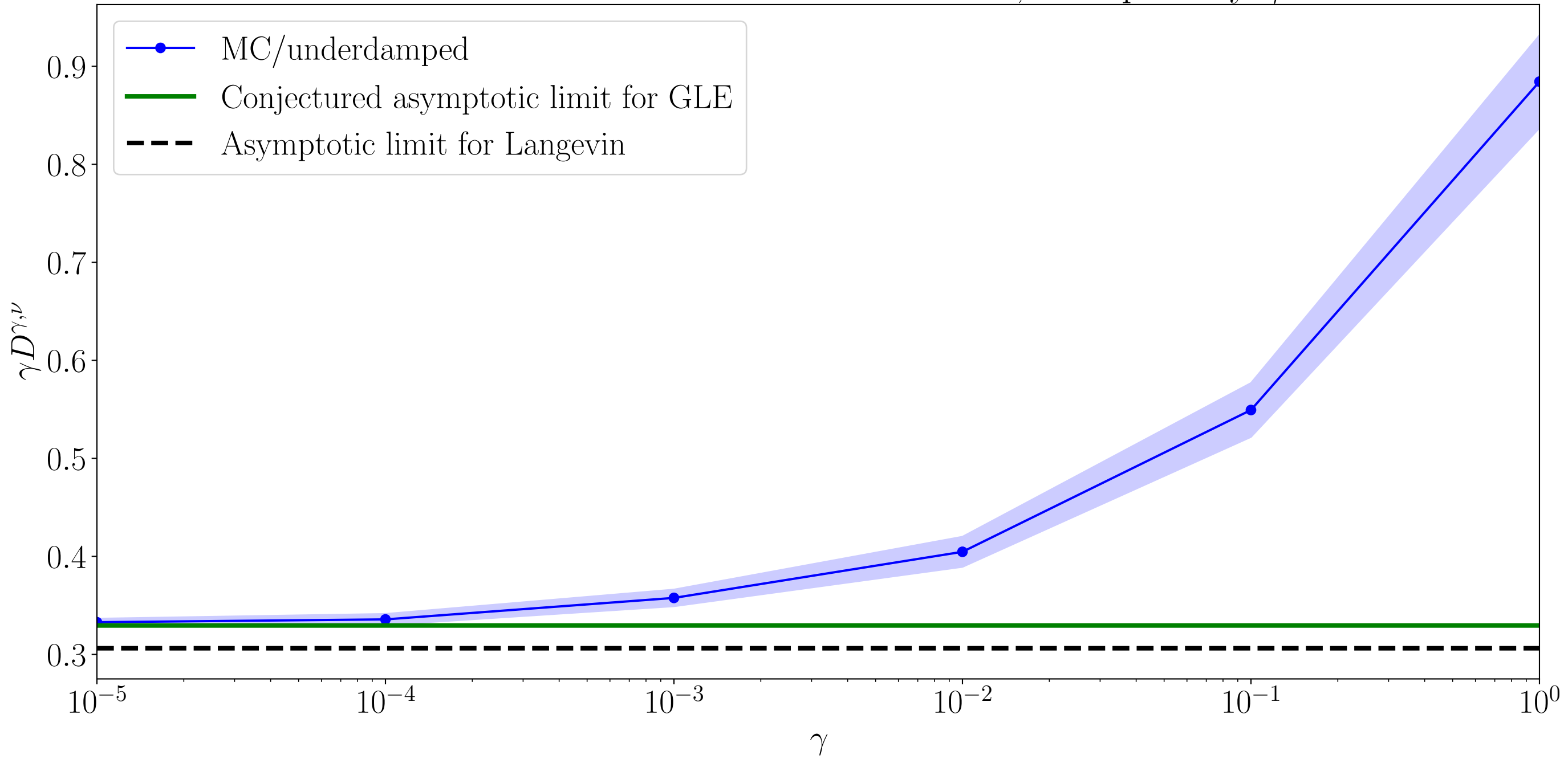
Effective diffusion coefficient for the GLE, multiplied by \gamma
