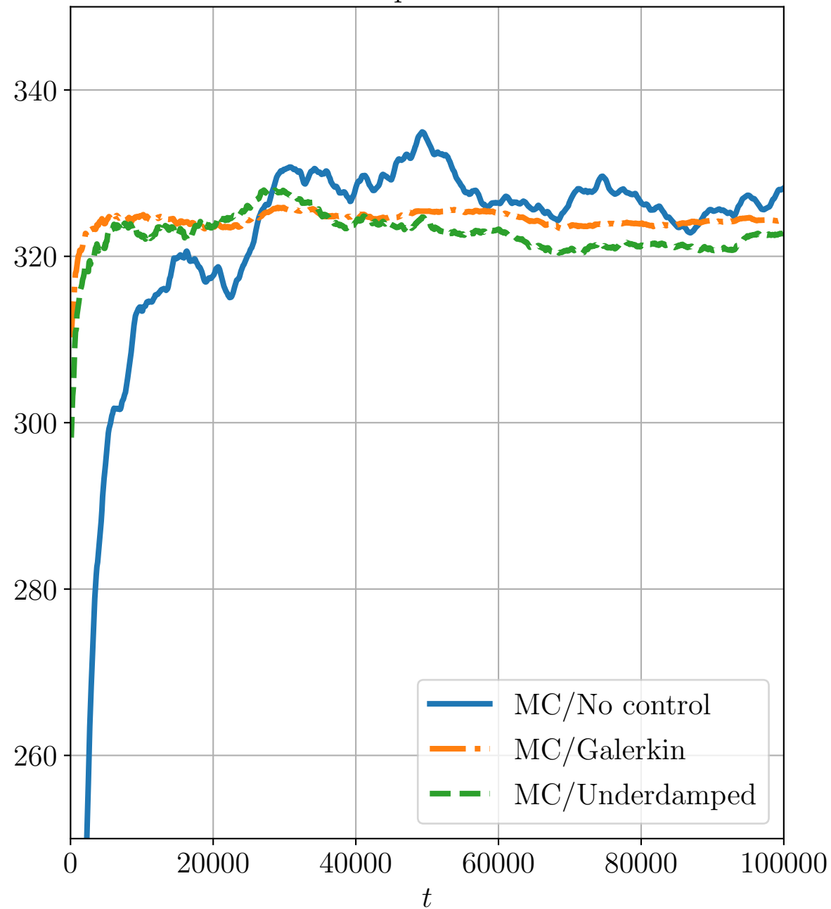
Sample mean
