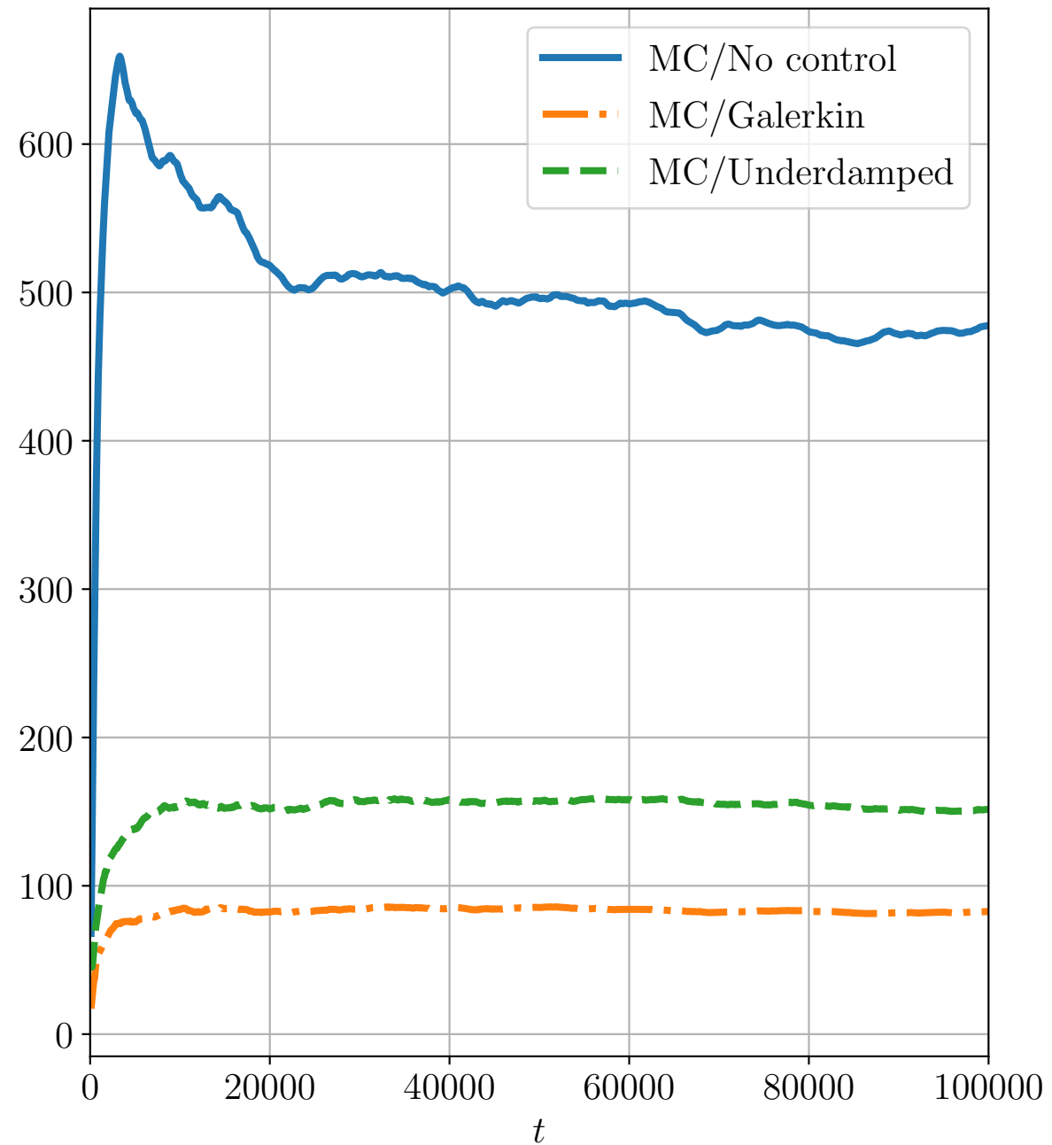
Standard deviation
